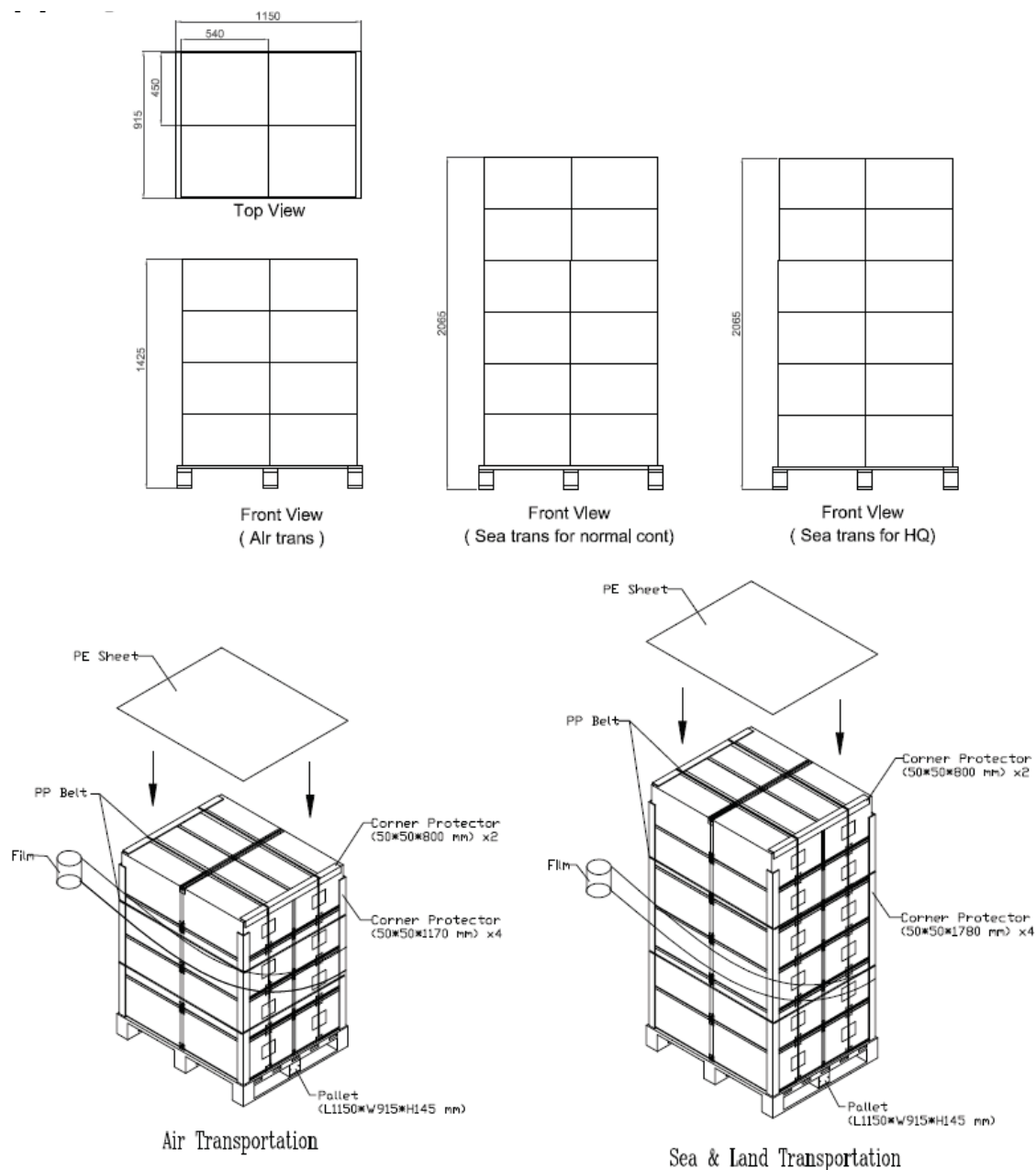
Figure. 7-3 Packing method
