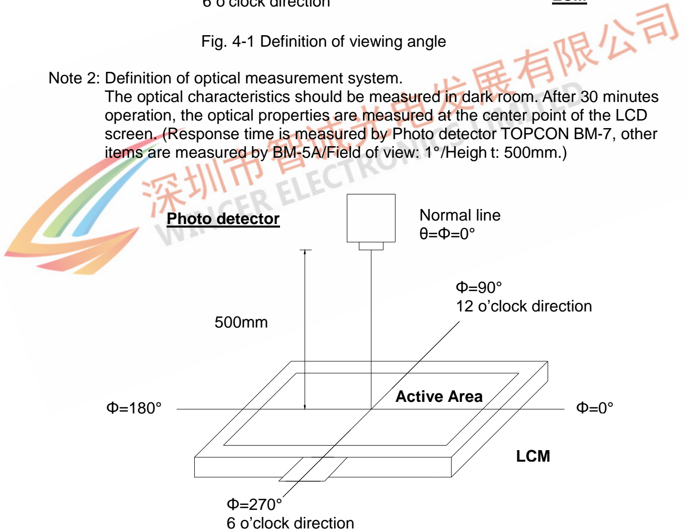
Fig. 4-2 Optical measurement system setup
