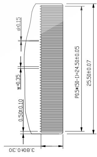
DETAIL A SCALE 4:1
